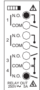
Quad Relay
