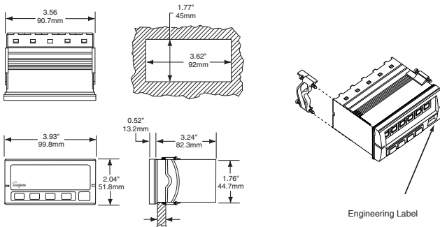
Figure 4-1. Installation and Panel Cutout
