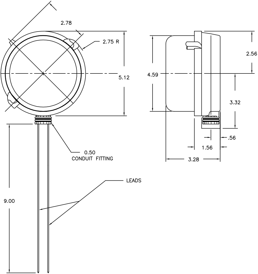
FIG. 24. OUTLINE DIMENSIONS FOR 240 TYPE CONDUIT-MOUNTED CASE REV 6/18/03 (DWG 3146K25)
