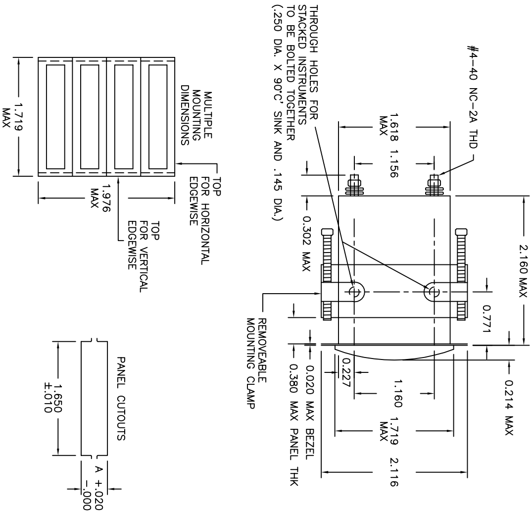
FIG. 17. OUTLINE DIMENSIONS FOR 1½ INCH TYPE 286 METERS REV 1/02/03 (DWG 3151K76)
