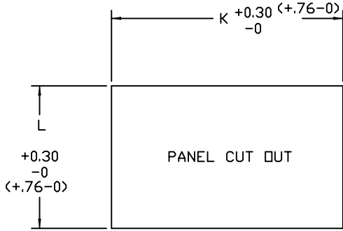
FIG. 10. STYLIST SERIES REV 4/1/03 BEZEL MOUNTS OF SURFACE MOUNT STYLIST METERS
